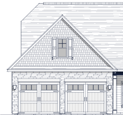
3 3'-0" WIDER GARAGE W/ TWO DOORS
